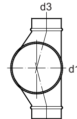
OBOK 90 exc.
